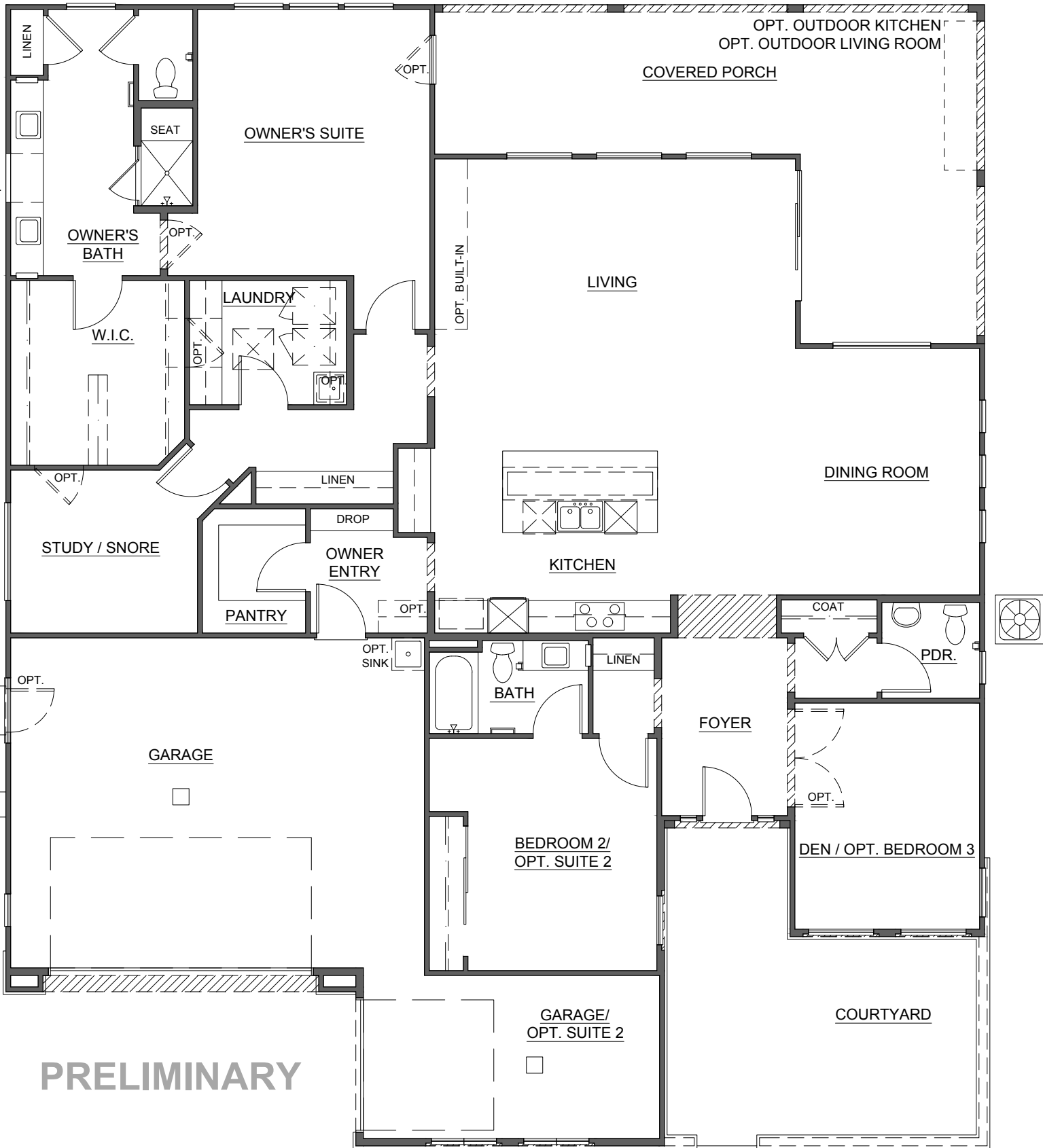
PLAN 60-3A | 2,499 S.F. | FLOORPLAN
